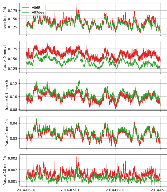
Figure 7: Time-series of IMERG V06B and V07 precipitation statistics over the ocean between 60°N/S in Jun–Aug 2014.
