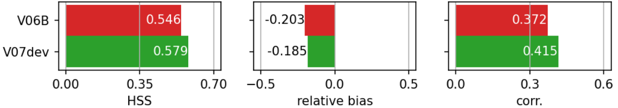
Figure 3: Evaluation of IMERG V06B precipitationCal and IMERG V07dev precipitation against GV-MRMS over the contiguous U.S. for Jun-Aug 2014.
