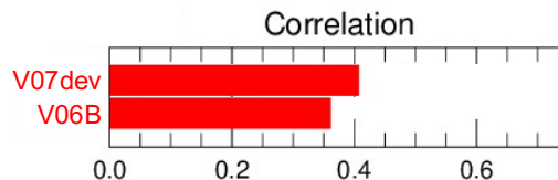
Figure 6: Correlation of IMERG V06B precipitation and IMERG V07 precipitation against KPOL over Jun–Aug 2014.
