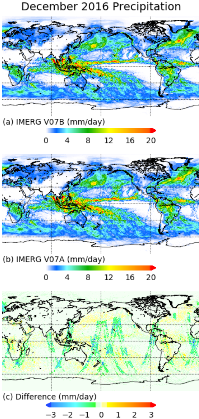
Fig. 8: Example of a) re-retrospectively processed IMERG V07B Final Run, b) the original retrospectively processed IMERG V07
